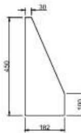
Stiffener 182 x 450 x 20mm Thick
