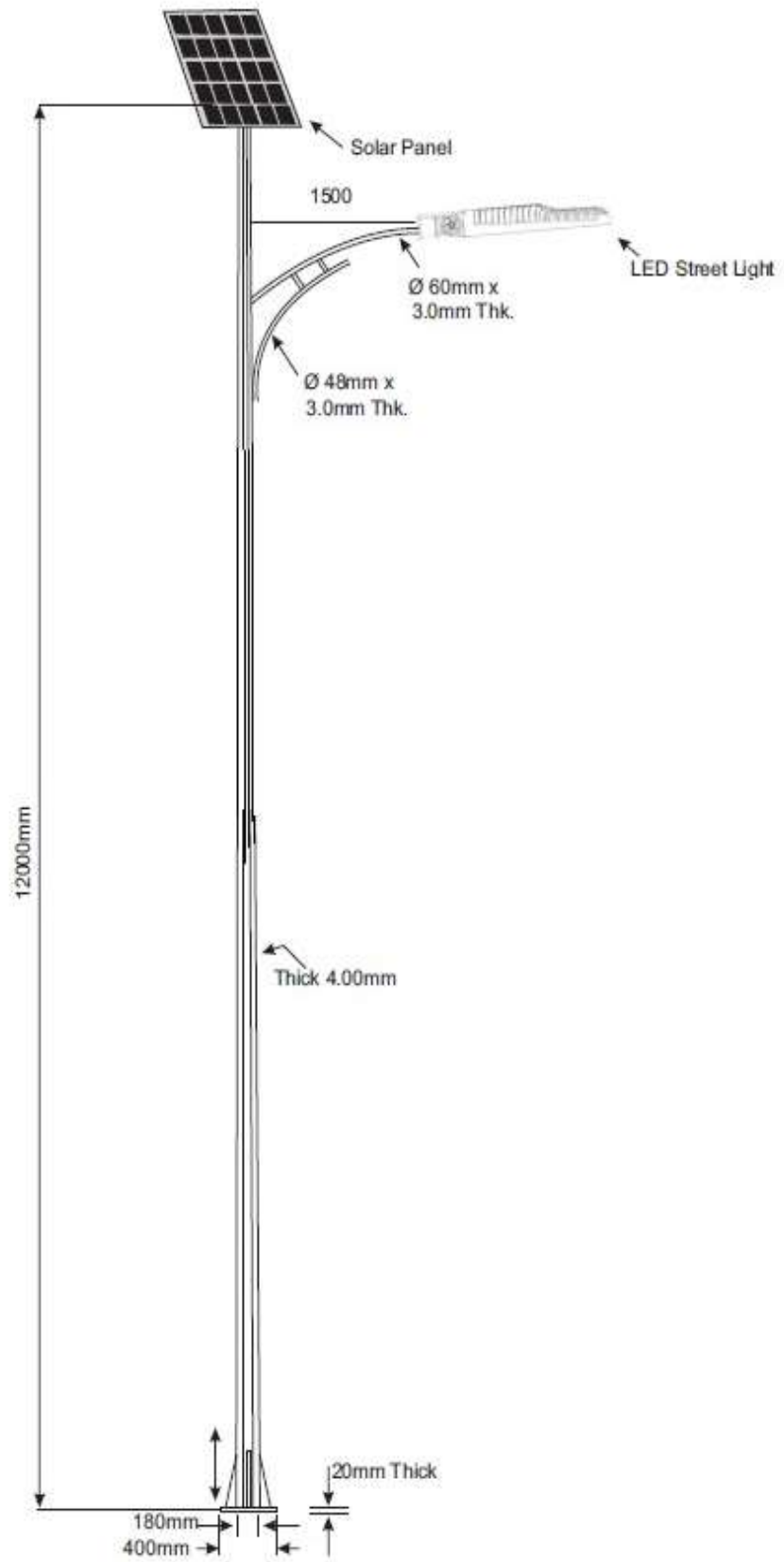
12-METERS POLE WITH SOLAR PANNEL
