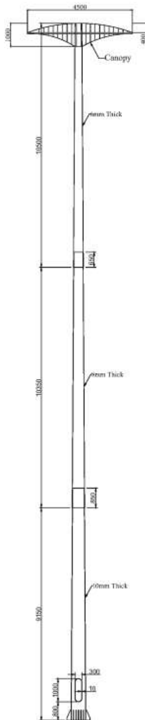
30M Polygonal (16 Sided) Flood Light Pole
