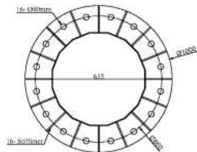
Base Plate Ø1000 x 35mm Thick
